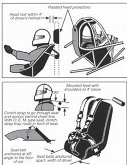
Figure 12 and 13: Head protectors and harness mounting
