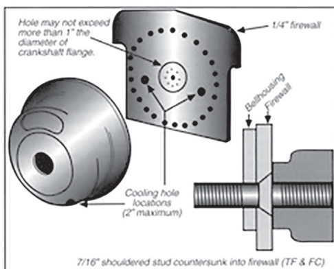
Figure 5: Motor Plate
