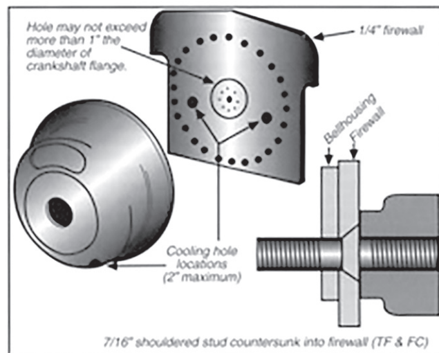
Figure 5: Motor plate
